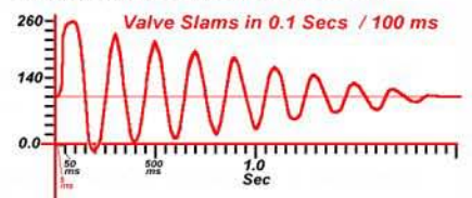
Rapid Valve Closure Hammer
